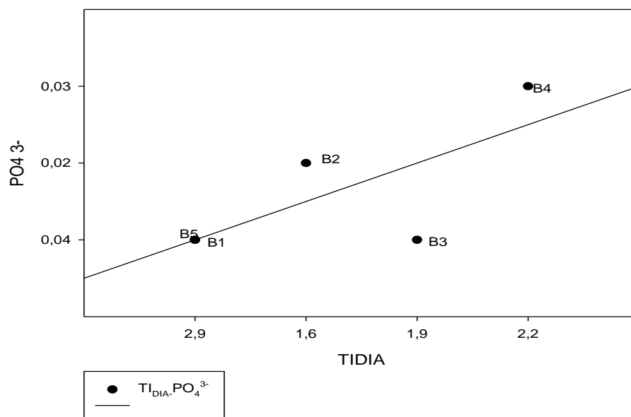
Figure 2. Correlation between Trophic Diatom Index ( TI_{DIA} ) and P-PO_4^{3-}
